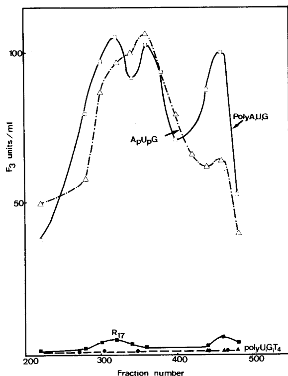
Fig. 3. Specificity of F3a towards different mRNAs. The amounts of fMet-tRNA bound by F1 + F2 were as follows with different mRNAs: poly A, U, G, 4.77; poly U, G, 1.148; ApUpG, 2.6; T 4 , 0.654; R17, 0.965. Binding conditions as in fig. 1 with 30 \mu l fractions of F3 (in 0.02 M buffer) containing between 1.5–3.4 \mu g protein.
